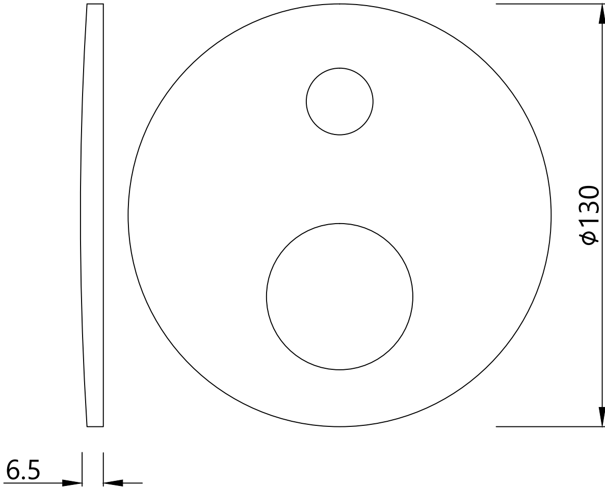
DIVERTER PLATE
