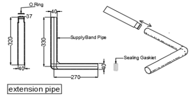
extension pipe
