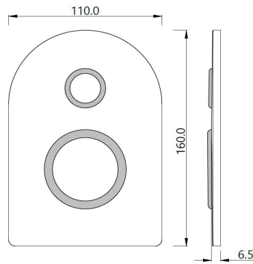
DIVERTER PLATE
