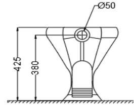
BACK VIEW
