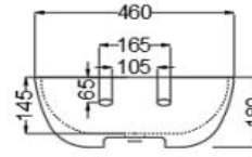
BACK VIEW
