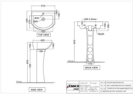
ECS-WHT-805 Wall Hung Basin with Full Pedestal
