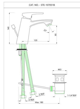
STE-CHR-107051B Single Lever Basin Mixer with Popup Waste
