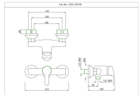
COS-CHR-103149 Single Lever Exposed Shower Mixer
