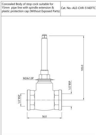
ALE-CHR-514EFTC Concealed Body of stop cock suitable for 15mm Pipe line
