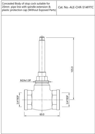
ALE-CHR-514FFTC Concealed Body of stop cock suitable for 20mm Pipe line
