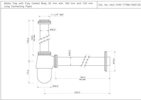
ALE-CHR-773ML190X125 Bottle Trap with Fully Casted Body
